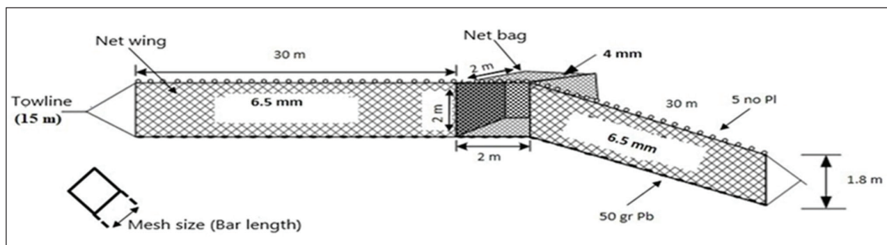
Fig. 2: Design and technical specifications of the beach seine net.
