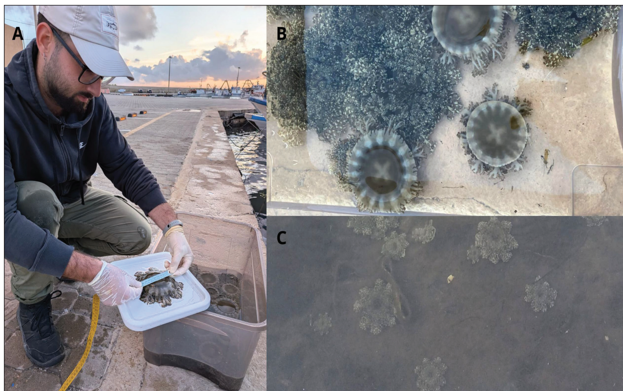
Fig. 1: Specimens of C. andromeda observed inside the harbour of Portopalo di Capo Passero (Sicily, Ionian Sea) on 19 October 2025: (A) during measurements; (B) sampled specimens; (C) in situ individuals.
